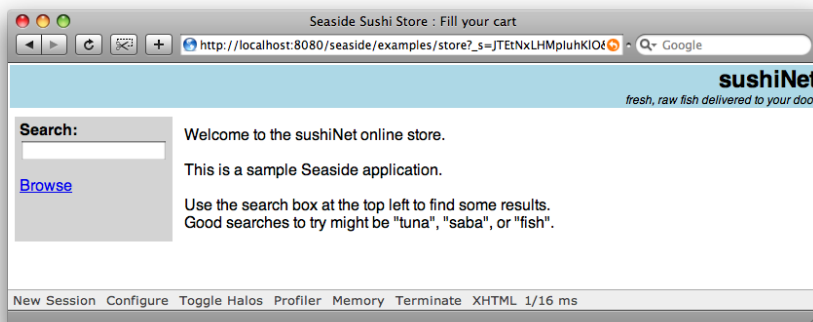
Figure 12.14: 寿司屋デモ
