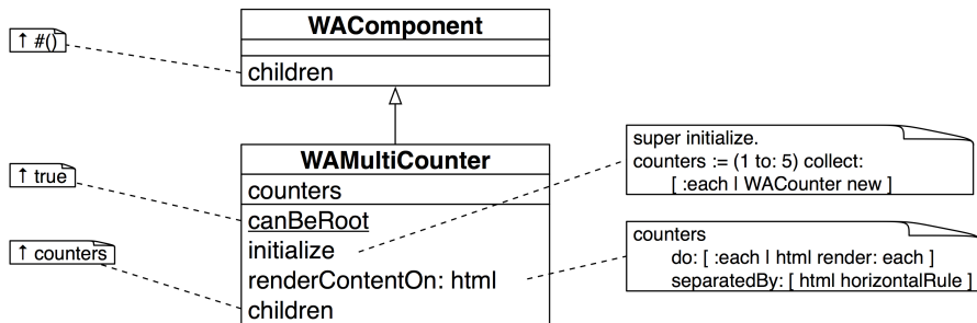
Figure 12.9: WAMultiCounter
