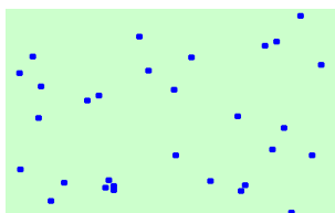
Figure 1.6: BouncingAtomsMorph。
