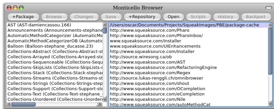
Figure 2.15: Monticello Browser.
