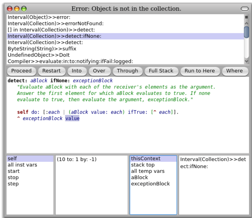
Figure 6.27: デバッガ
